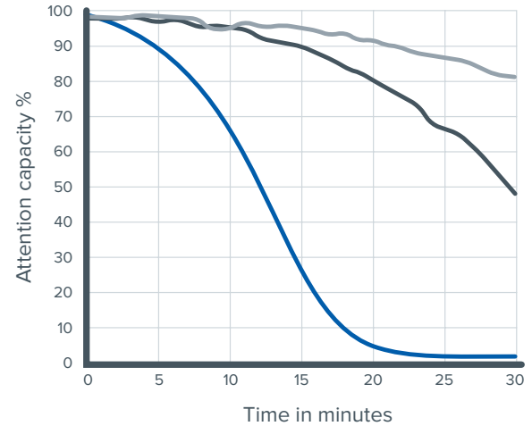
Pattern Detection
